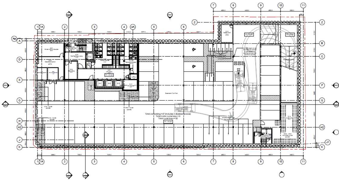
LEVEL -1 PLAN - Basement 1:100
