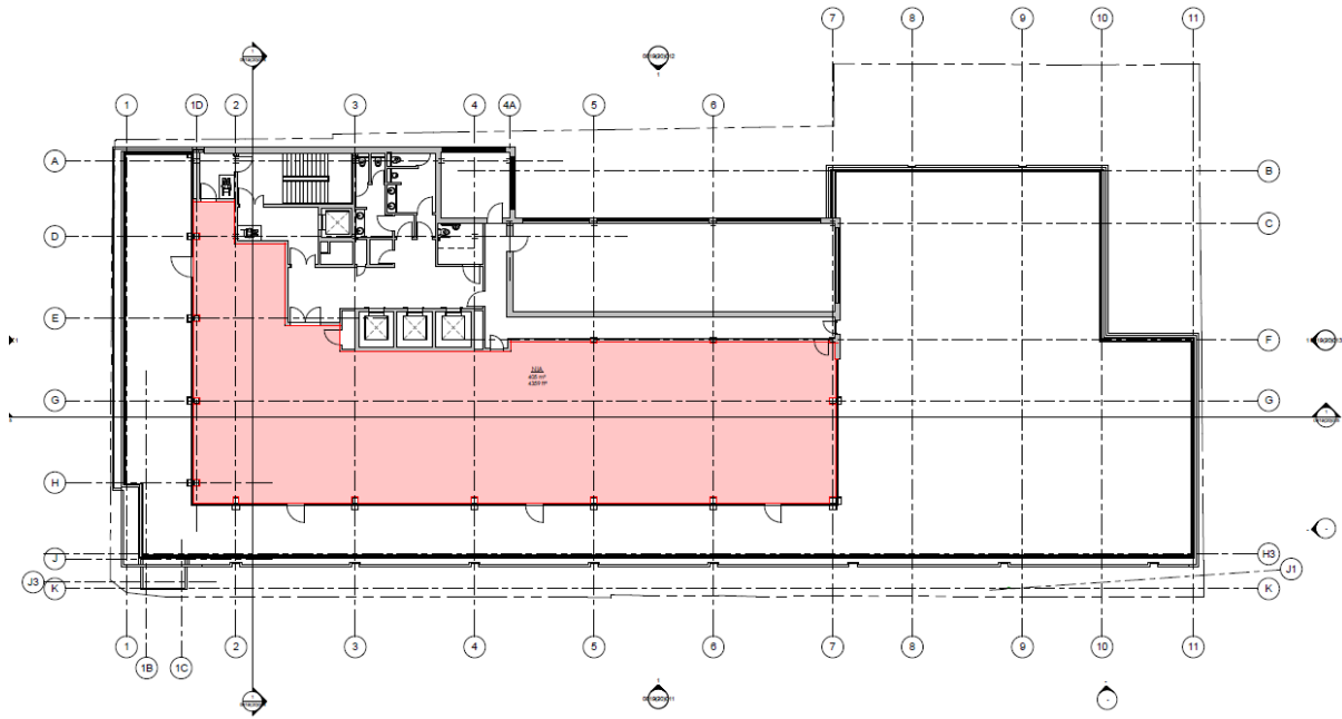
LEVEL +5 PLAN - Fifth Floor NIA 1:100
