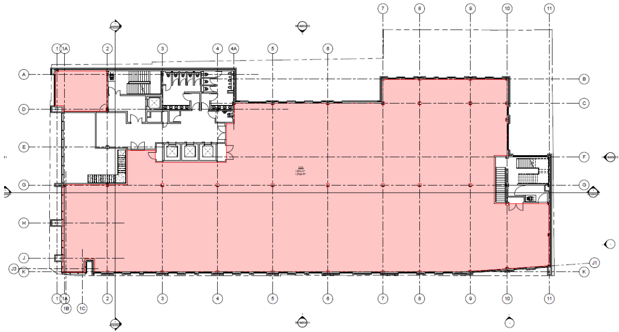
LEVEL +1 PLAN - First Floor NIA 1:100
