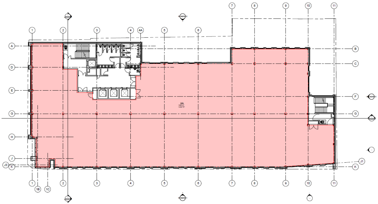
LEVEL +03 PLAN - Third Floor NIA 1:100
