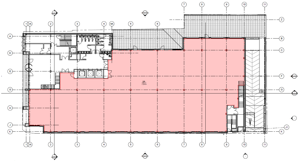
LEVEL +0 PLAN - Ground Floor NIA 1:100
